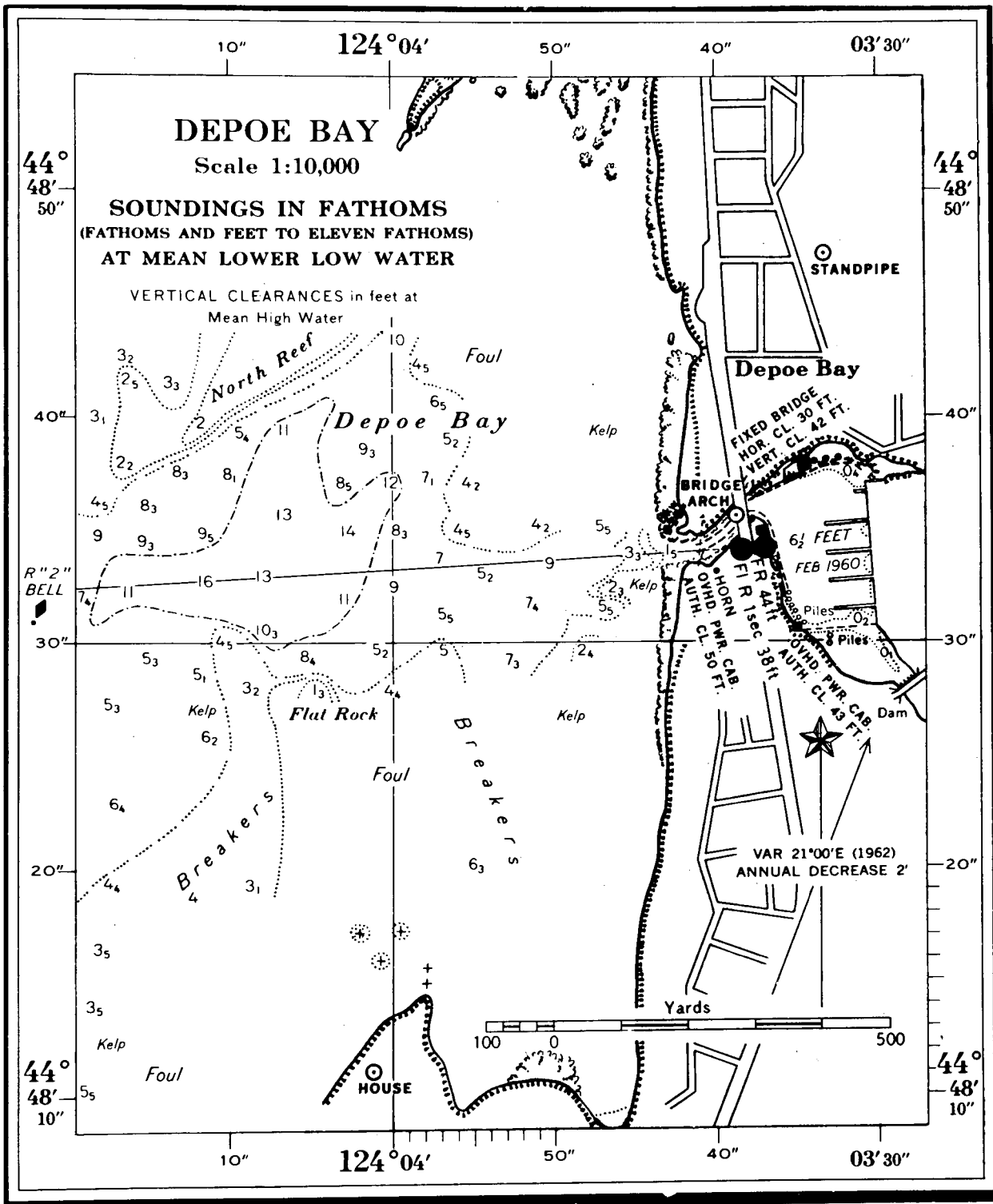
Fig. 9. Outer and inner harbors of Depoe Bay.
